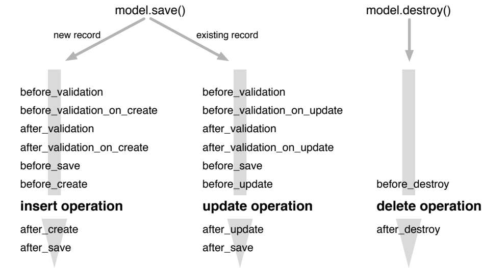
Figure 19.2: Sequence of Active Record callbacks
