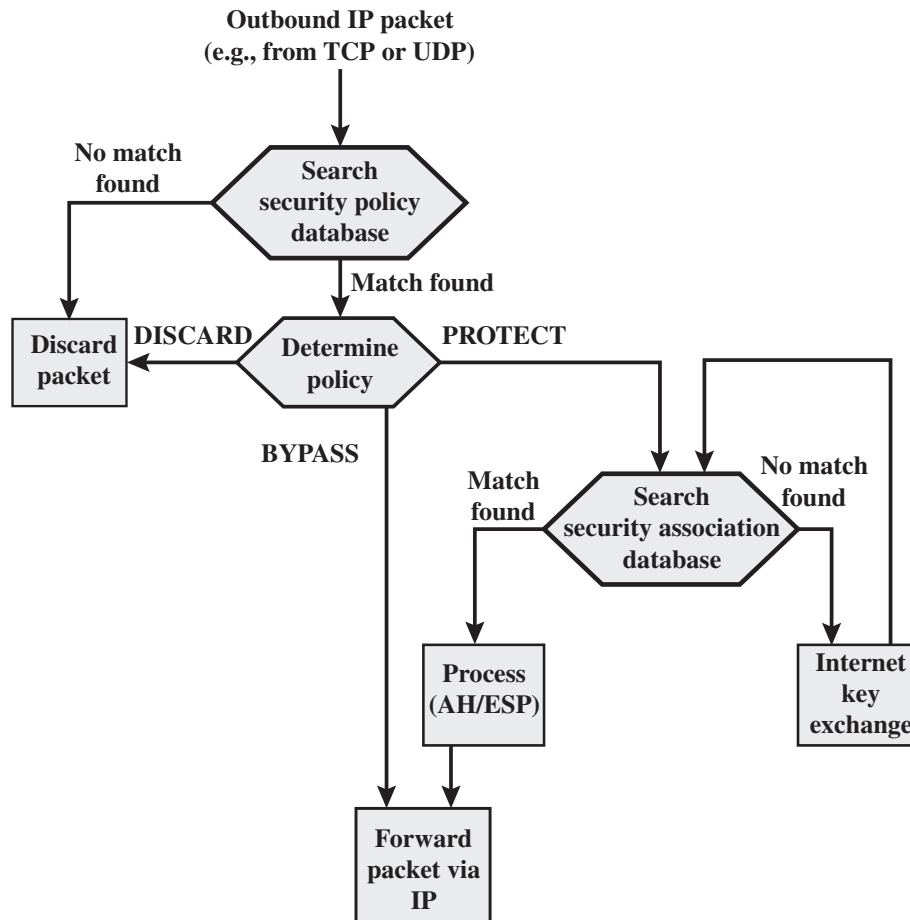
Figure 8.3 Processing Model for Outbound Packets
