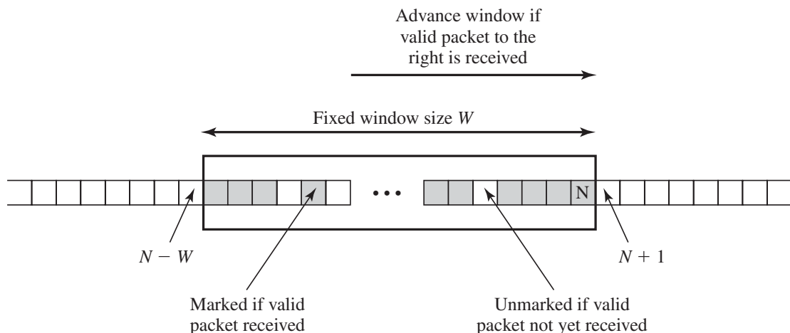
Figure 8.6 Anti-replay Mechanism
