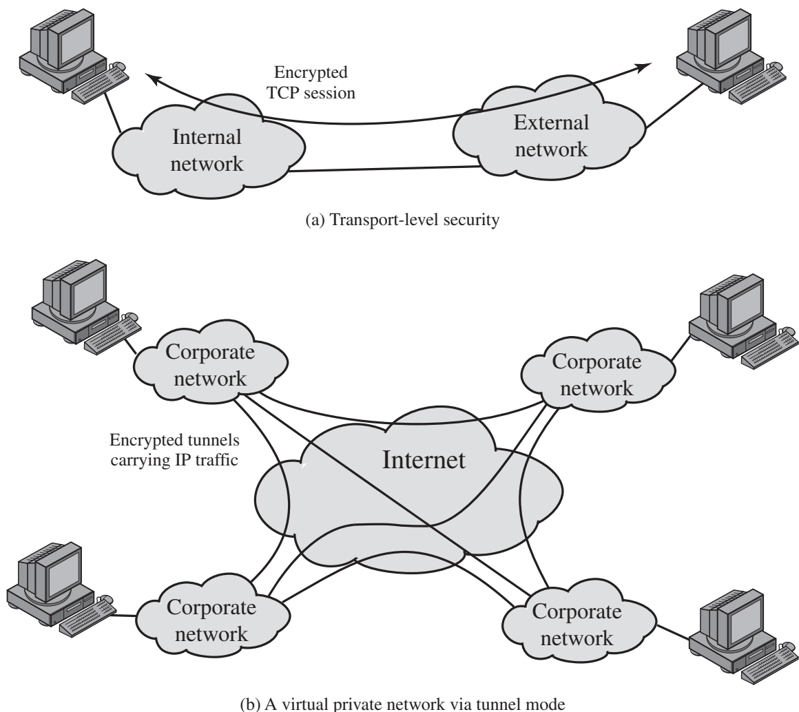
Figure 8.7 Transport-Mode versus Tunnel-Mode Encryption
