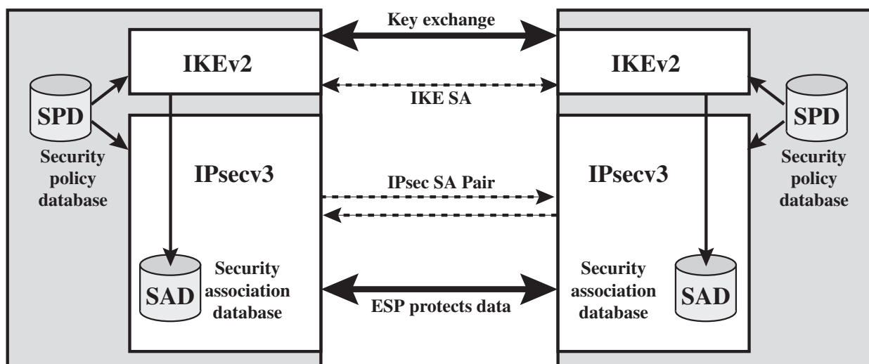
Figure 8.2 IPsec Architecture
