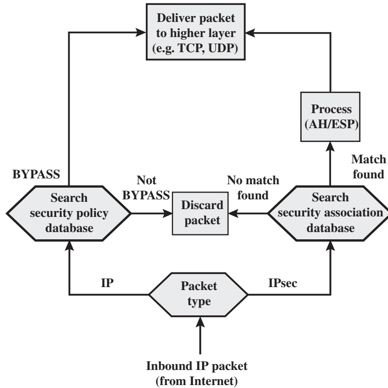
Figure 8.4 Processing Model for Inbound Packets
