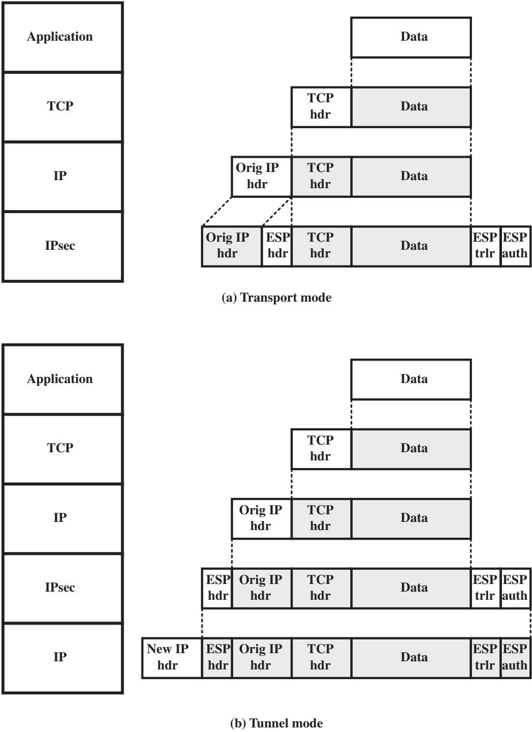
Figure 8.9 Protocol Operation for ESP
